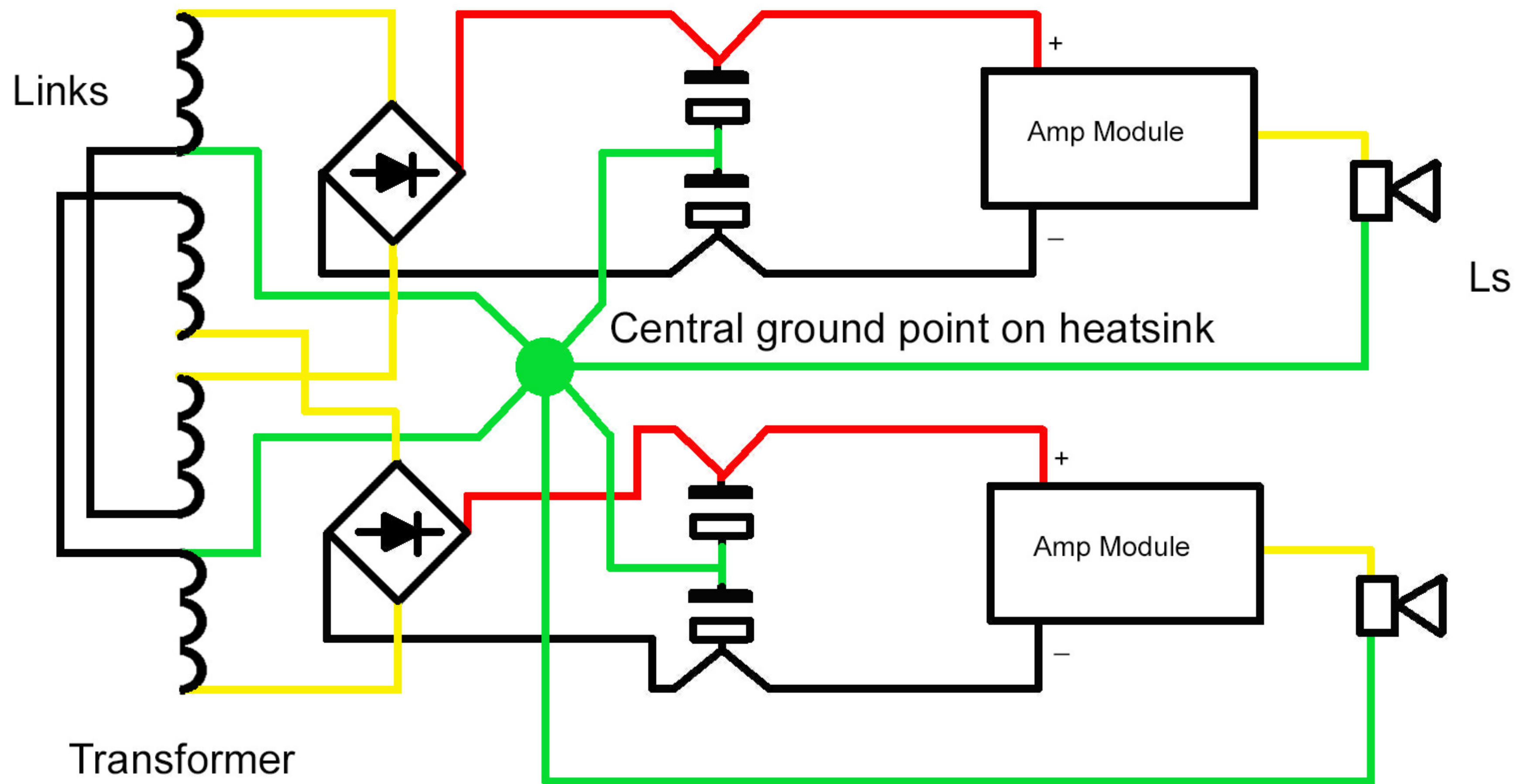
Quad 405 dual and normal supply wiring diagrams
